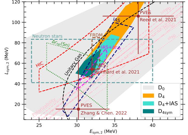
FIG. 6. Same as Fig. 1 including the new contours from the present analysis: D_4 , D_4+IAS , D_{4sym} . The light-grey band represent the contour of all explored interactions (group D_0=G_0 ).
