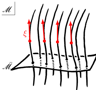
Figure 2. A principal \mathbb{R} -bundle (\mathcal{M} \rightarrow \bar{\mathcal{M}}, \xi) . Each curve is a fibre, and all points of that fibre are mapped by the projection (3.1) on a single point on the base \bar{\mathcal{M}} . The bundle \mathcal{M} is locally isomorphic to a product \bar{\mathcal{M}} \times \mathbb{R} , but in the case at hand this is even true globally, thanks to the global existence of a smooth (\mathbb{R}, +) group action.
