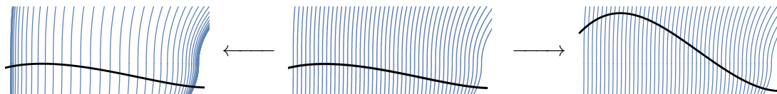
Figure 3. Given the bundle \mathcal{M} \rightarrow \bar{\mathcal{M}} , any bundle automorphism maps \bar{\mathcal{M}} to itself smoothly, but generally shuffles its points so that different fibres are mapped on one another (left). Furthermore, automorphisms locally change the origin of the Carrollian time coordinate (right). They also affect the local normalisation of the fundamental vector field (not shown here). In the BMS context, local translations along fibres are supertranslations, while superrotations are automorphisms projecting onto conformal maps of the base space: see sections 3.3–3.4.
