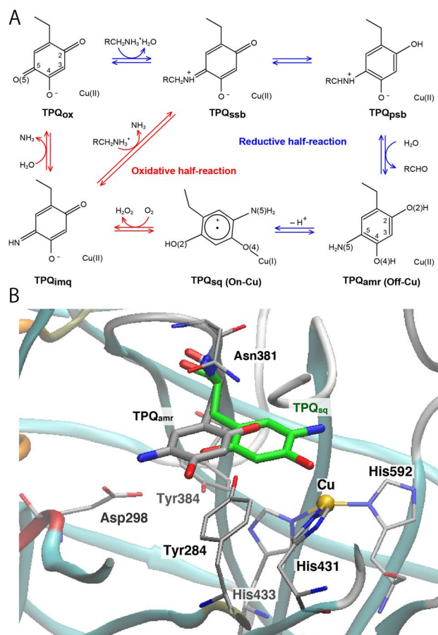
Fig. 1 (A) The proposed catalytic cycle of AGAO 14 . The stable and intermediate states are the oxidized form (TPQ ox ), the substrate Schiff base (TPQ ssb ), the product Schiff base (TPQ psb ), the aminoresorcinol (TPQ amr ), the semiquinone radical (TPQ sq ), and the iminoquinone (TPQ imq ). Among all these, only TPQ sq is detected in the on-copper conformation. (B) The conformational changes of TPQ in the aminoresorcinol and semiquinone radical states. TPQ amr is located away from the Cu coordination site (off-copper), while TPQ sq , colored in green, approaches the Cu site (on-copper). Two X-ray crystal structures of AGAO are superimposed (PDB ID: 3X3X, 3X3Z) 14 .
