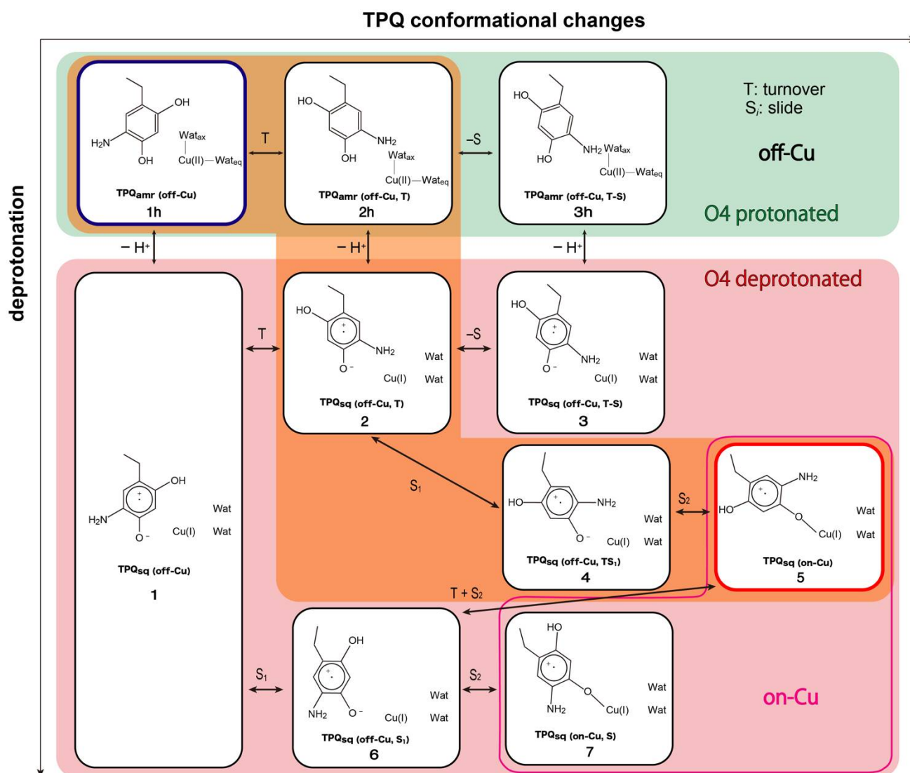
Fig. 4 A comprehensive view of the intermediate states on which the present work is focused for the TPQ ammr to TPQ sq transition. The letter “h” added in the labeling as in 1h–3h stands for the protonated state on O4-TPQ. The orange background highlights the main reaction pathway, whereas the green background refers to the O4-TPQ protonated state, and the red one does the deprotonated one.
