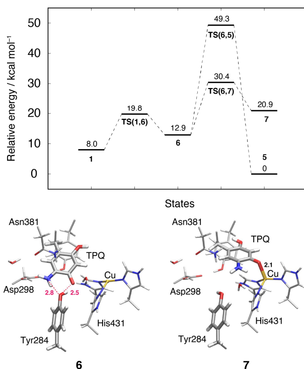
Fig. 7 Relative energies of alternative TPQ conformational changes in the deprotonated state, including the TPQ slide motion ( 1 → 6 → 7 ) and the rotation ( 6 → 5 ). The conformations of the intermediate states are reported along with the most relevant distances between heavy atoms.
