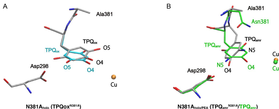
Fig. 3 X-ray structures of the holo N381A crystal in the TPQ ox and TPQ amr conformations. The TPQ rings are flipped in both states. (A) The TPQ ring-flipped conformation of TPQ ox N381A is colored by element, in which the non-ring-flipped conformation is colored in cyan. (B) The N381A structure of TPQ amr is superimposed to the WT structure (PDBID: 3X3Z) 14 , colored in green for a direct comparison.
