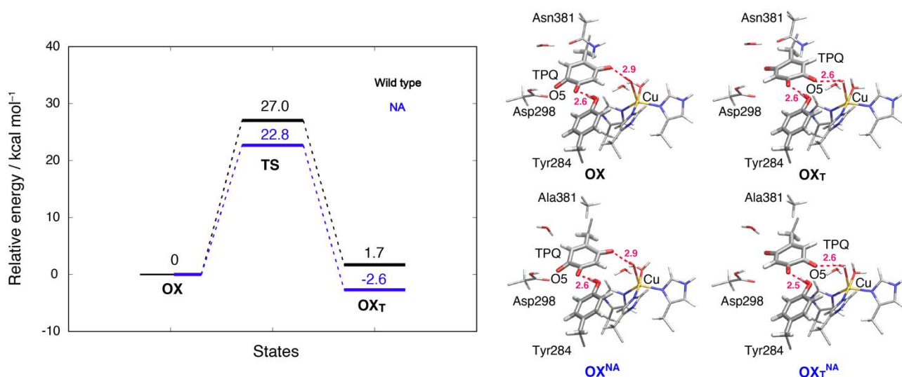
Fig. 8 Relative energies and related conformations for the TPQ rotation in the oxidized form. Results for the WT and the N381A mutant are shown in black and blue, respectively. Most relevant distances between the heavy atoms are explicitly indicated.
