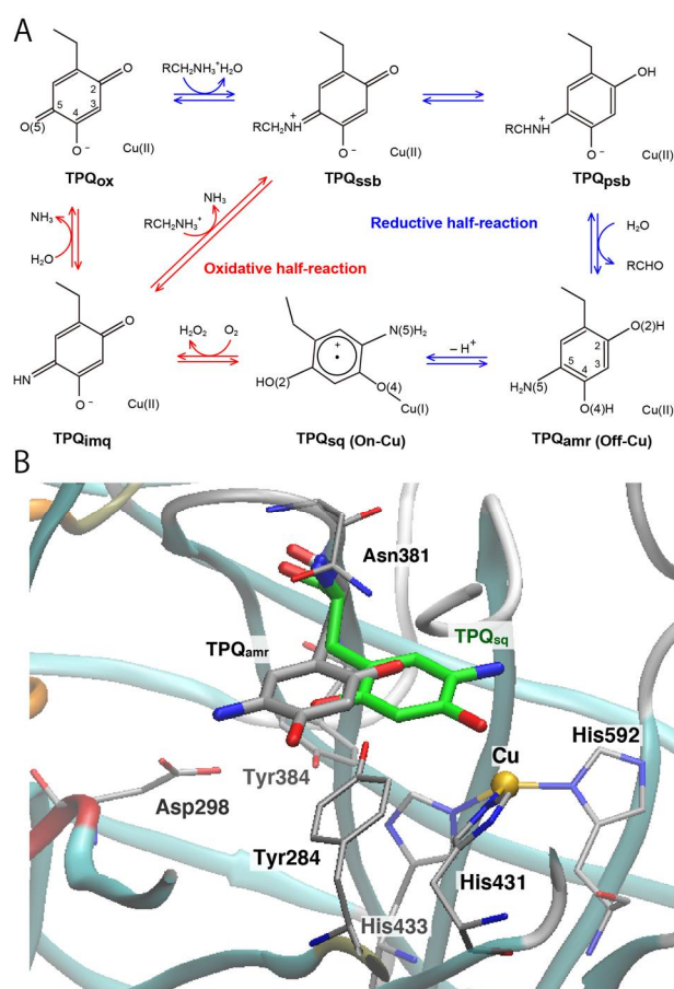
Fig. 1 (A) The proposed catalytic cycle of AGAO 14 . The stable and intermediate states are the oxidized form (TPQ ox ), the substrate Schiff base (TPQ ssb ), the product Schiff base (TPQ psb ), the aminoresorcinol (TPQ amr ), the semiquinone radical (TPQ sq ), and the iminoquinone (TPQ imq ). Among all these, only TPQ sq is detected in the on-copper conformation. (B) The conformational changes of TPQ in the aminoresorcinol and semiquinone radical states. TPQ amr is located away from the Cu coordination site (off-copper), while TPQ sq , colored in green, approaches the Cu site (on-copper). Two X-ray crystal structures of AGAO are superimposed (PDB ID: 3X3X, 3X3Z) 14 .
