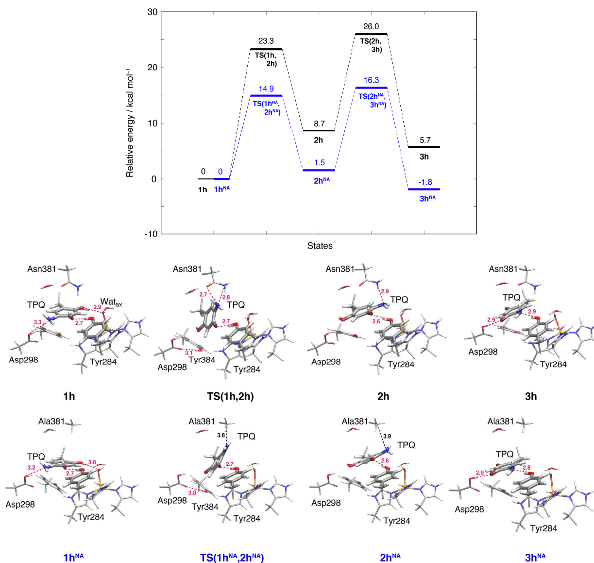
Fig. 5 Relative energies associated with the TPQ conformational change in the protonated state. Results for the WT and the N381A mutant (NA) are shown as black and blue lines, respectively. Molecular structures of the intermediate and transition states are reported with the most important distances between heavy atoms.
