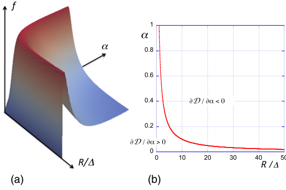
FIG. 13. Diffusion suppression: (a) general shape of function f(\alpha, R/\Delta) with 0 < \alpha < 1 , 1 < R/\Delta < 50 . (b) Crest line separating the region of diffusion suppression ( \partial\mathcal{D}/\partial\alpha > 0 ) from region \partial\mathcal{D}/\partial\alpha < 0 .
