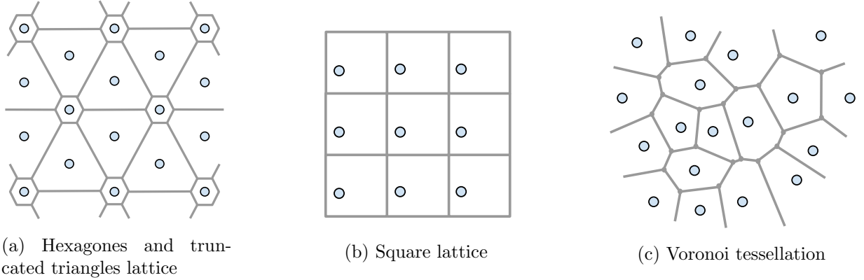
Figure 1: Three examples of tilings in \mathfrak{T}^2 (see Definition 1.2) with a particular choice of reference points shown as light-blue circles. The resulting structures are point-referenced 2-honeycombs.
