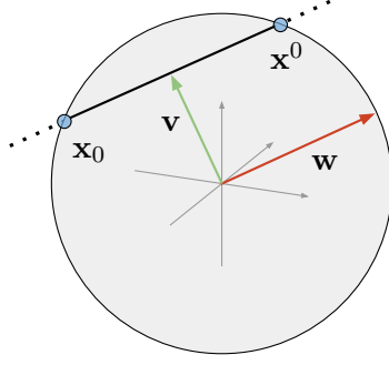
Figure 3: In dimension 3, the unit ball is represented; the red vector is a possible \mathbf{w} \in \partial B_1^3 and the green vector, a possible \mathbf{v} \in \text{vect}(\mathbf{w}^\perp) \cap B_1^3 . The two endpoints \mathbf{x}_0 and \mathbf{x}^0 , marked in blue, describe the segment \overline{l_{\mathbf{w},\mathbf{v}}} .
