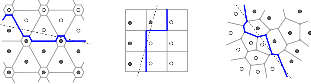
Figure 2: For each of the point-referenced 2-honeycombs in Figure 1, a portion of the level curve \{X = u\} is illustrated as a dotted line. The estimator \hat{C}_d^{(\mathcal{H}, T)}(u) in (10) corresponds to the length of the resulting blue curve that separates the reference points in the same way as the curve \{X = u\} .
