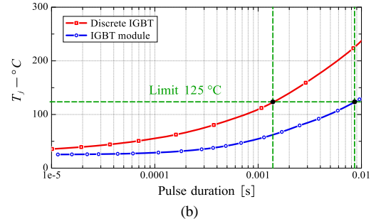
Fig. 6 (a) Thermal resistance from junction to case for discrete IGBT and IGBT module, (b) relationship between T_j and duration of 1 kA pulse current.
