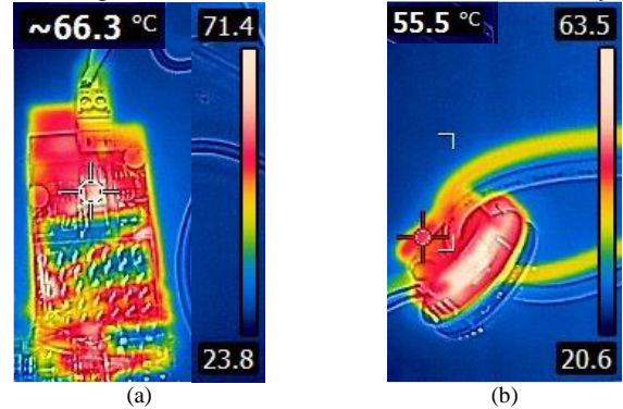
Fig. 19 Thermal test results of (a) primary board and (b) 20 W secondary circuit.
