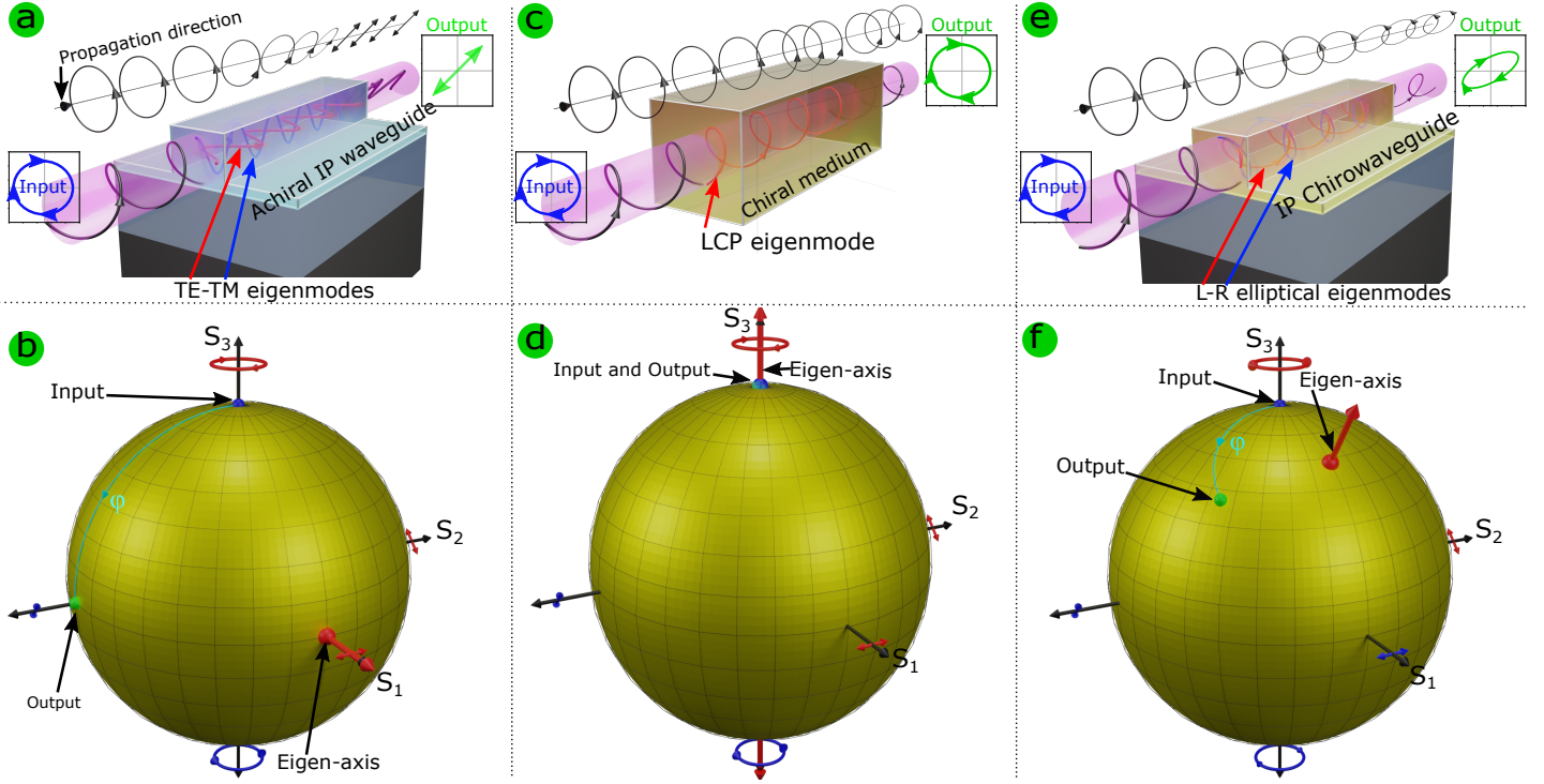
Figure 1: Concept of polarized wave transformation in birefringent systems in real space (a,c, and e) and Poincaré sphere (b,d, and f). An input polarized wave propagating through these systems decomposes into two orthogonal polarized waves called eigenmodes. In Poincaré sphere (PS), the two eigenmodes create a diameter axis (eigen-axis) in which the birefringence effect on any input wave other than the eigenmodes is a rotation of the input around the eigen-axis. The value of rotation angle ( \varphi ) depends on interaction length ( l ) and the difference of effective refractive indices of the two eigenmodes ( \Delta n ). In Poincaré sphere, \varphi give by eq.5, here, (lMB/\lambda) = \lambda/4 then \varphi = 2\pi in which the achiral waveguide behaves as a quarter waveplate. a-b ) IP waveguides made of standard (achiral) materials are linear birefringence systems. TE/TM are their two eigenmodes ( \pm S_1 ). c-d ) Chiral media are circular birefringence systems. R/L CP are their two eigenmodes ( \pm S_3 ). Combination of linear (IP) and chiral birefringence results into e-f ) IP chirowaveguides which are elliptical birefringence systems. Their eigenmodes are between TE/TM and R/L-CP which is defined by eq. 4.
