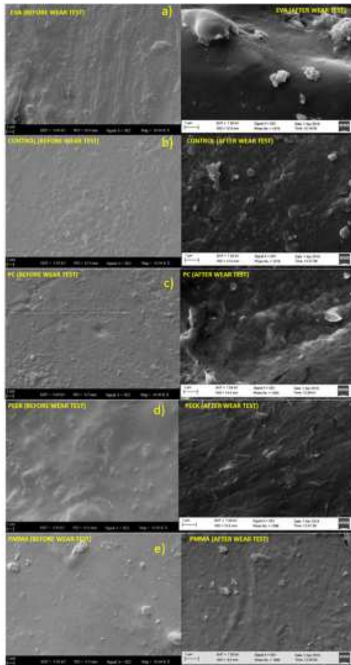
Figure 3. SEM images of the group samples before and after the wear test (a) EVA (Ethylene Vinyl Acetate), (b) C (PETG- Polyethyleneterephthalate), (c) PC (Polycarbonate), (d) PEEK (Polyetheretherketone), (e)PMMA (Polymethyl methacrylate)(magnification 10000x)
