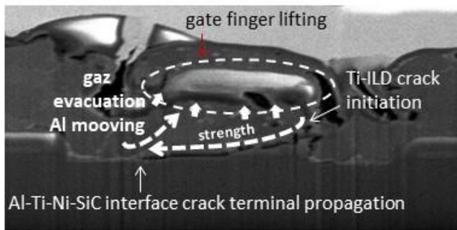
b) A-MOSFET 1.2kV gate finger lift-off highlighting moving by strength crack and Al melting – gaz.
