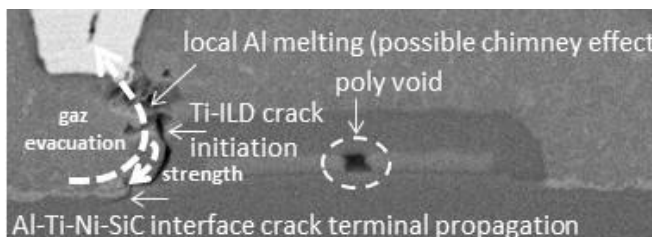
b) A-MOSFET 1.2kV gate finger lift-off highlighting moving by strength crack and Al melting – gaz.
