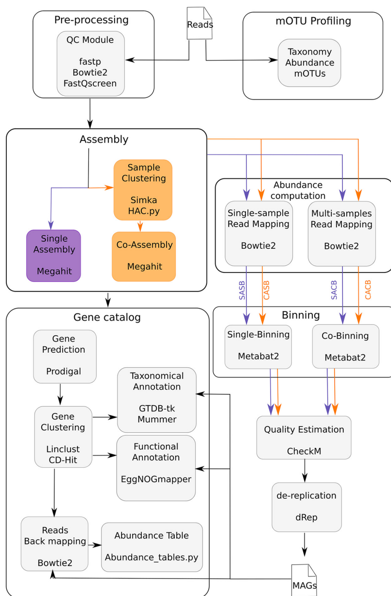
FIG 5 Overview of the MAGNETO workflow summary view of modules implemented in the MAGNETO workflow, with the name of the software or script associated with each task. The workflow can be launched for a complete run, to process raw reads into a gene catalog and MAGs, but each module can also be run independently. In purple: path to perform single assembly, corresponding to SASB (single assembly single binning) and SACB (single assembly cobinning) strategies, and orange: path to perform coassembly, corresponding to CASB (coassembly single binning) and CACB (coassembly cobinning) strategies.
