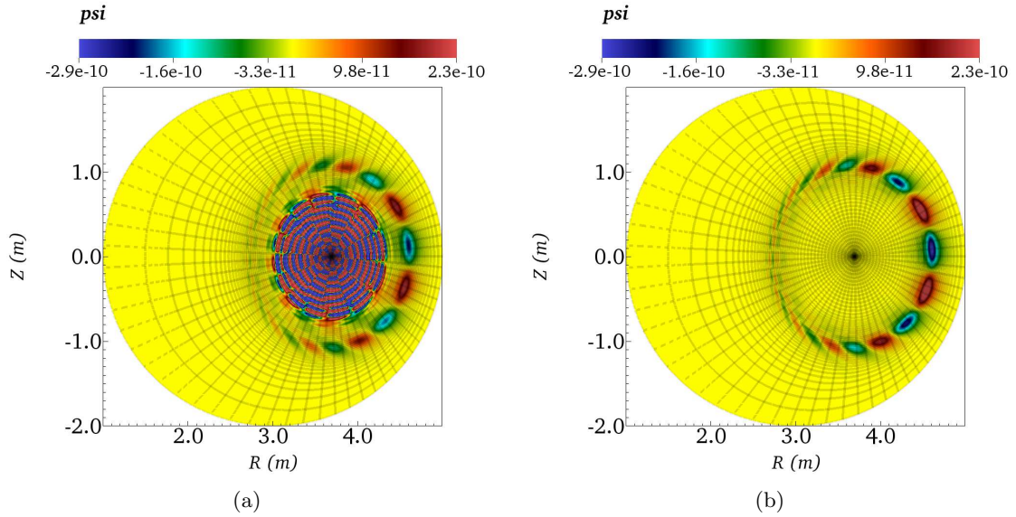
Figure 16: Circular ballooning mode instability structures in the magnetic flux \psi = R A_\phi for n = 6 with the a) intermediate and b) C^1 polar treatment obtained on the Grid 0 from Figure (14).
