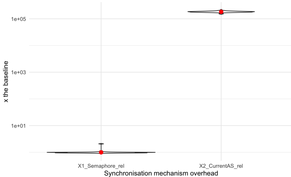
Figure 3: Overhead induced by synchronisation mechanisms in current Pharo implementation:
