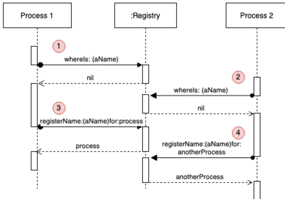
Figure 1: Order for bad message interleavings. 1. Process 1 checks first if the name is registered and spawns a new process. 2. Process 2 does the same. 3. Process 1 registers a process with the name. 4. Process 2 also spawns and tries to register a process with the same name instead of throwing an error.
