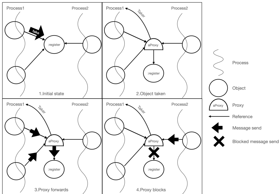
Figure 2: Example of Atomic Samurai with two processes.
