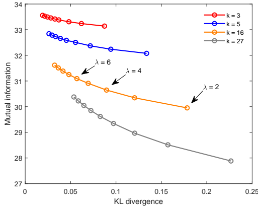
Figure 11: Performance of correlated sparse attack construction in linearized AC model in terms of mutual information and KL divergence for different values of \lambda on the IEEE 9-bus system with \text{SNR} = 30 dB and \rho = 0.9 .
