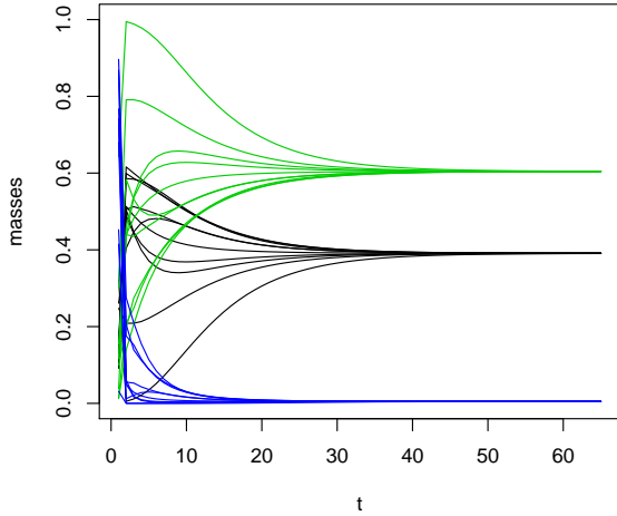
Fig. 5. Convergence of masses m_i(\{\omega_1\}) , m_i(\{\omega_2\}) and m_i(\{\Omega\}) to the orthogonal sum, for the static consensus mechanism.
