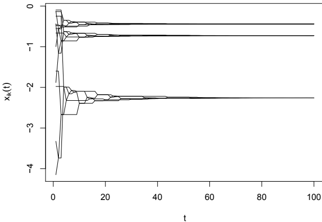
Fig. 3. Convergence of state variables x_{ik}(t) to the averages \alpha_k for the dynamic consensus mechanism.
