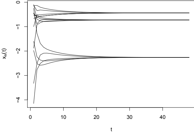
Fig. 2. Convergence of state variables x_{ik}(t) to the averages \alpha_k for the static consensus mechanism.
