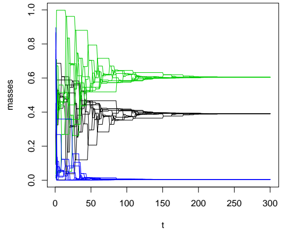
Fig. 7. Convergence of masses m_i(\{\omega_1\}) , m_i(\{\omega_2\}) and m_i(\{\Omega\}) to the orthogonal sum, for the dynamic (symmetric gossip) consensus mechanism.
