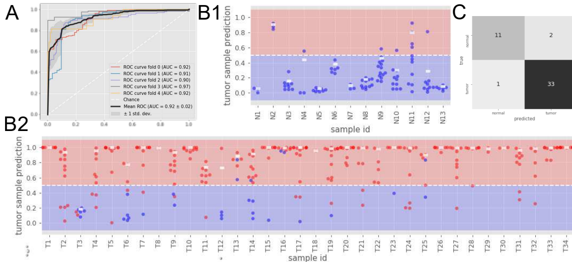
Figure 3: CNN classification of breast cancer (A) ROC curves and AUCs of the 5-fold cross validated models. (B) Tumor probability prediction by the CNN for each ROI in each sample, either healthy (B1) or tumoral (B2). Each point represents a ROI which ground truth diagnosis is either healthy (blue) or tumoral (red). The white rectangle represents the aggregated tumor probability per sample, computed as the 90th percentile of the probabilities of the ROIs in a sample : (B1) normal samples prediction (B2) tumoral samples prediction.
