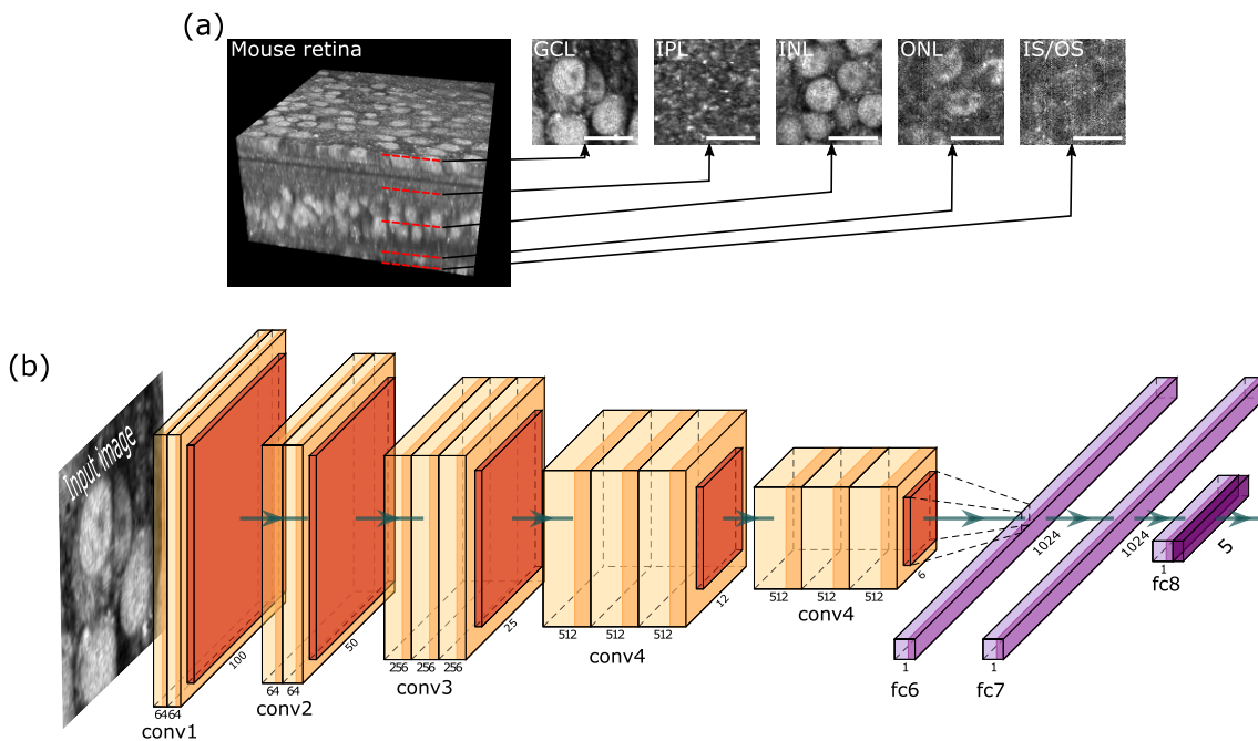
Figure 8: (a) 3D stack of mouse retina on 80 \mu\text{m} depth. 697 thumbnail images of 100 \times 100 pixel (corresponding to 27 \times 27 \mu\text{m} ) were randomly selected and manually classified on a single retina in 5 different classes: GCL, IPL, INL, ONL and IS/OS. (b) Neural network architecture based on VGG16 used for classifying thumbnail images in 5 different classes. Only the last fully connected layers (depicted in purple) were trained. Scale bar: (a) 25 \mu\text{m} .
