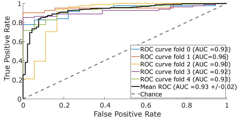
Figure 9: AUC Curves linear SVM
