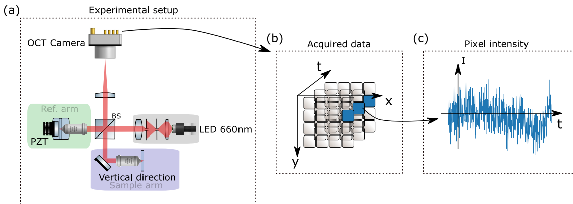
Figure 5: PZT: piezoelectric translation - BS: Beam splitter. Experimental D-FFOCT setup in an inverted configuration optimized for tissue imaging. 512 images are acquired by the CMOS camera (a). The resulting (1440, 1440, 512) 3D tensor (b) is then processed independently for each pixel (c).
