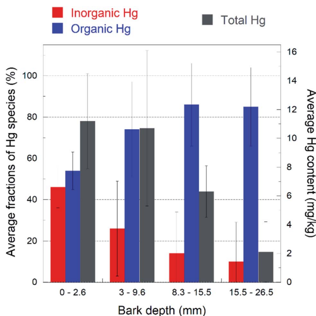
Fig. 4 Bar plot highlighting the trend of the inorganic (nano- \beta\text{HgS} , red color) and Hg-organic (blue color) fractions (%) as a function of the depth of the bark layer. Total Hg content ( \text{mg kg}^{-1} ) is also reported (gray color). The fractions shown are the averages of the values reported in Table S1.† for each layer. The bark layer thicknesses have been averaged, because they were slightly different for each bark sample (see the Materials and methods). The data show that the organic Hg fraction increases with depth at the expense of the inorganic one, and the total Hg content decreases with depth. The error bars represent the standard deviations for each layer ( n = 5 ).
