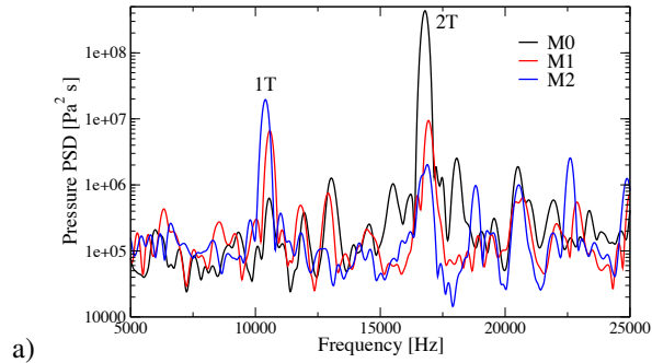
Figure 5: Case T131. Power spectral density of pressure in (a) the chamber and (b) the LOx post for cases M0, M1 and M2. A Welch's method with 1 block is used, df=200 Hz, the last 5 ms are used for each case.
