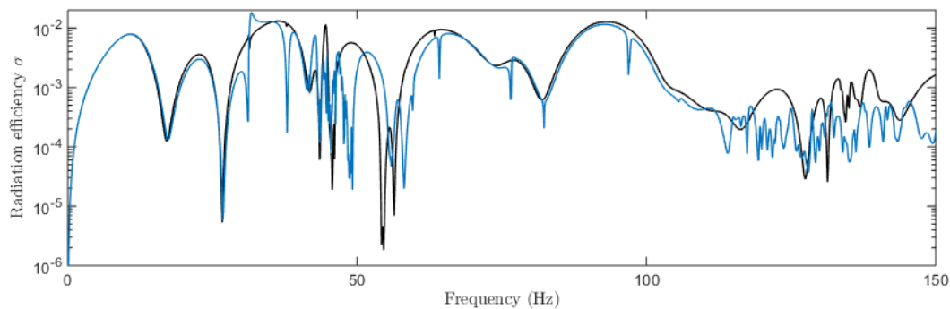
Figure 6: Radiation efficiencies obtained with the FE method: (black solid line) purely periodic plate; (blue solid line) nearly periodic plate.
