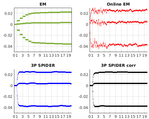
Fig. 3 Estimation of three parameters. Evolution of the three components of \theta by EM in green (top, left), OEM in red (top, right), 3P-SPIDER in blue (bottom, left) and 3P-SPIDER corr in black (bottom, right), as a function of the number of epochs.
