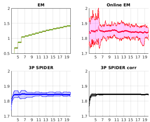
Fig. 4 Squared norm of the iterates. Evolution of \|\hat{S}_r^{\text{EM}}\|^2 in green (top, left), \|\hat{S}_r^{\text{OEM}}\|^2 in red (top, right), \|\hat{S}_{t,k}\|^2 for 3P-SPIDER in blue (bottom, left) and \|\hat{S}_{t,k}\|^2 for 3P-SPIDER corr in black (bottom, right), as a function of the number of epochs.
