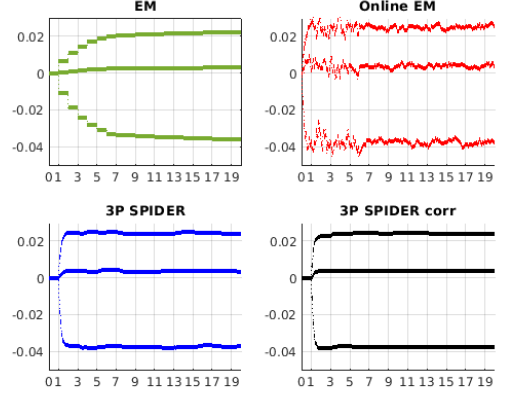
Fig. 3 Estimation of three parameters. Evolution of the three components of \theta by \Delta_r^{\text{EM}} in green (top, left), \Delta_r^{\text{OEM}} in red (top, right), \Delta_{t,k+1} for 3P-SPIDER in blue (bottom, left) and \Delta_{t,k+1} for 3P-SPIDER corr in black (bottom, right), as a function of the number of epochs.
