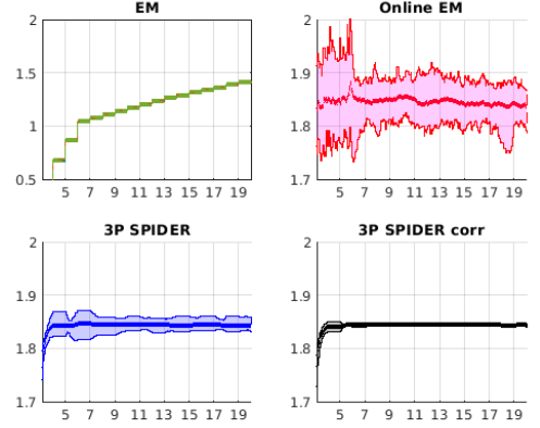
Fig. 4 Squared norm of the iterates. Evolution of \|\hat{S}_r^{\text{EM}}\|^2 in green (top, left), \|\hat{S}_r^{\text{OEM}}\|^2 in red (top, right), \Delta_{t,k+1} for 3P-SPIDER in blue (bottom, left) and \Delta_{t,k+1} for 3P-SPIDER corr in black (bottom, right), as a function of the number of epochs.
