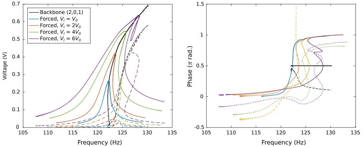
Fig. 8 Amplitudes and phases of the forced responses around the (2, 0, 1) mode, plot with colors, with V_0 = 62\text{V} . The amplitudes and phases of the signals V_{s1} and V_{s2} are, respectively,
