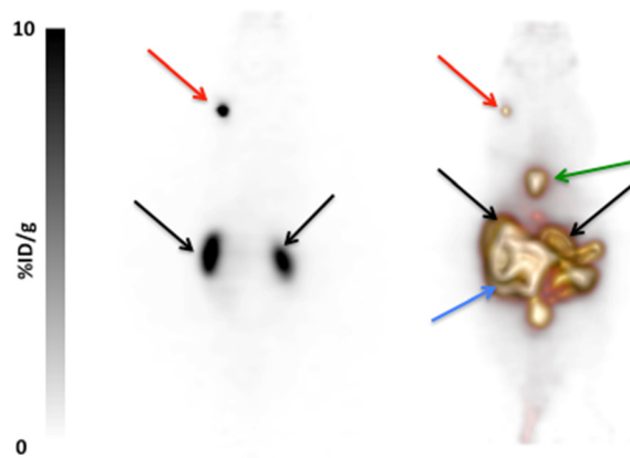
Fig. 2 Left: Anterior coronal view of a mouse bearing an LNCap tumor 60 min after i.v. injection of 10 MBq of [ ^{18}\text{F} ]- 11 ; red arrows point to the tumor, black to the kidneys. Scale bar from 0 to 10% ID \text{g}^{-1} for the left image. Right: Anterior view of whole-body 3D volumic rendering of the same mouse; green arrow for gallbladder and blue for the intestines.
