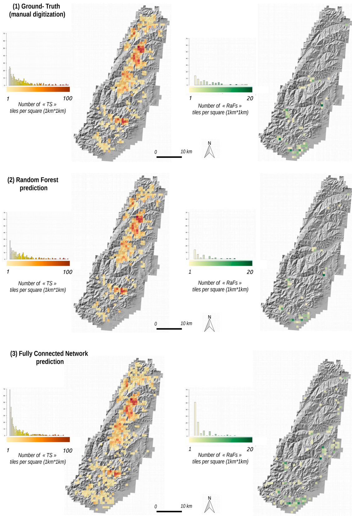
Fig. 8. Prediction maps of TS and RaF over the entire study site for the different detection models against validation maps. Predicted positive tiles (128 m × 128 m) were summed for each 1 km × 1 km cell. Colour gradients illustrate positive tile variations over cells, whereas histograms show cell densities according to their number of positive tiles.
