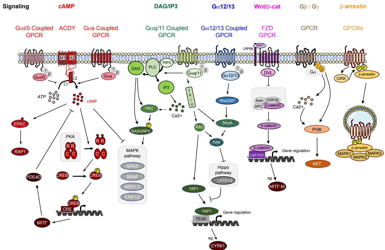
Figure 1. GPCR signaling pathways. Note that the G\alpha_{q/11} et G\alpha_{12/13} G-proteins share a common downstream signaling intermediate—YAP1.
