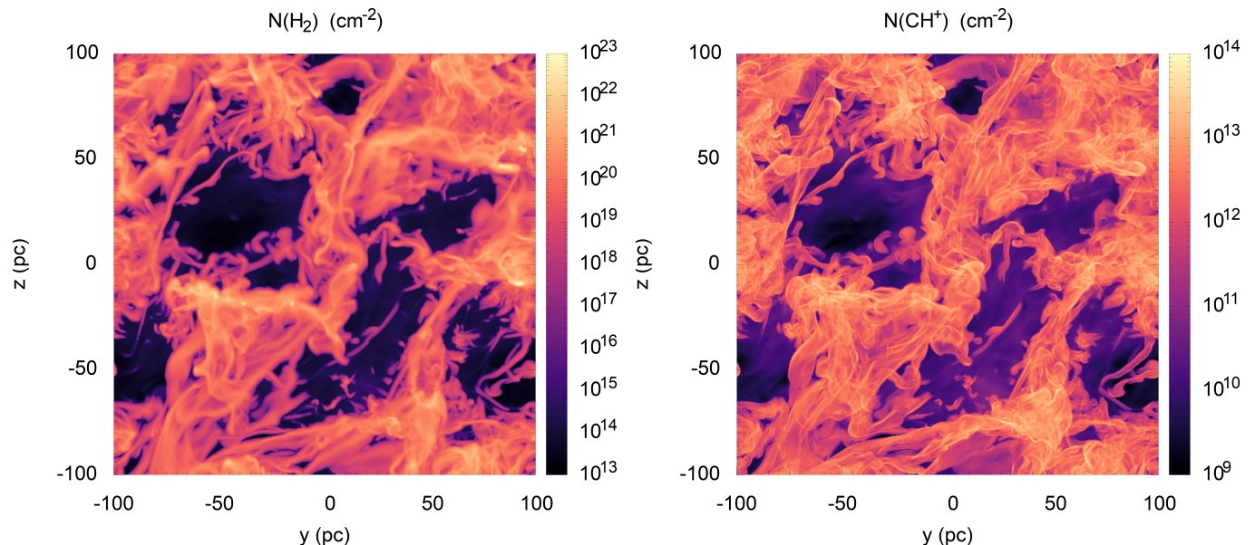
Fig. 4. Maps of the column densities of H 2 (left panel) and CH + (right panel) predicted with the standard simulation (see Table 1) and obtained by integrating the densities along the x axis over the entire box of size L = 200 pc.
