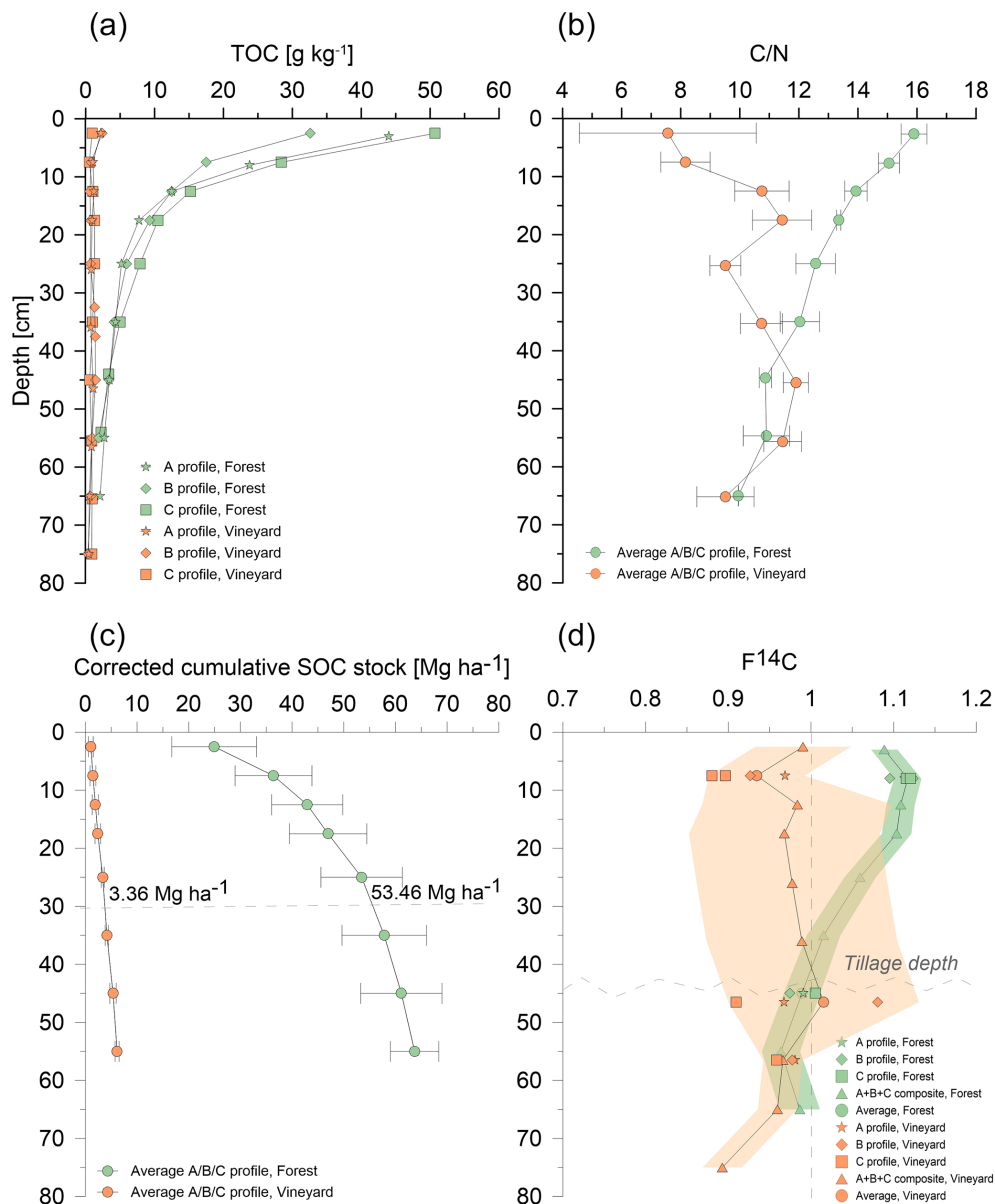
Figure 2. TOC variations (a), C : N ratio (b), cumulative stocks corrected for equivalent mass (c), and F 14 C profiles (d) as a function of depth, under vines (orange) and under forest (green), for an Arenosol under a Mediterranean climate. The corrected cumulative SOC stocks error bar represents the standard deviation. The F 14 C measurement variability (d) is represented by green (forest) and orange (vine) bands.
