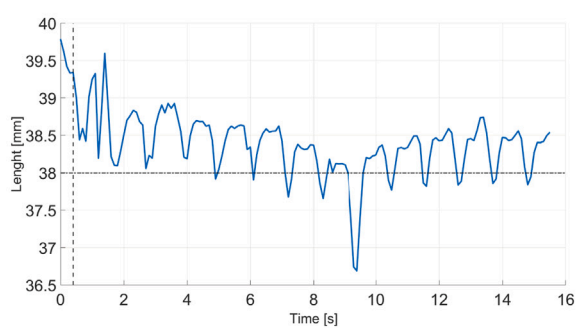
(d) Measurement of layer with 38 [mm] width.
