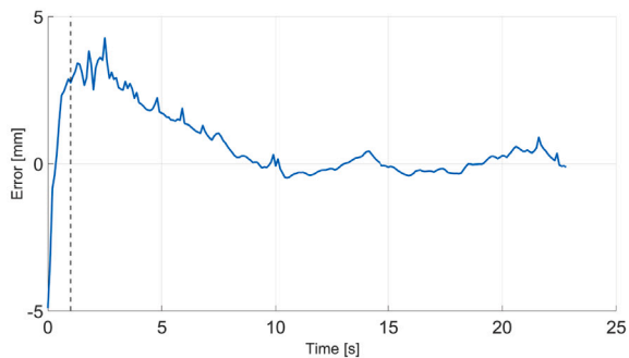
(b) Error on layer with 42 [mm] width.
