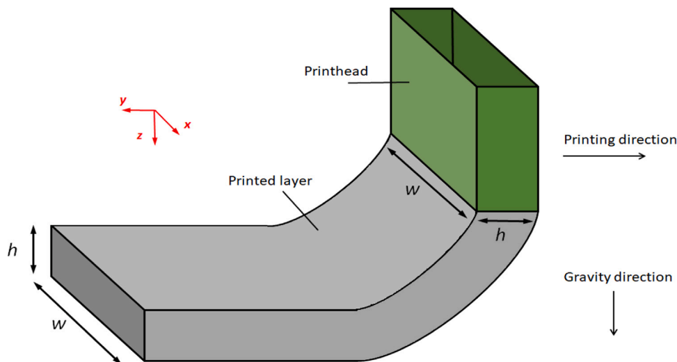
Fig. 1. Schematic drawing of extrusion of a very stiff material (infinite brick strategy) which creates layers with individual height h and width w .
