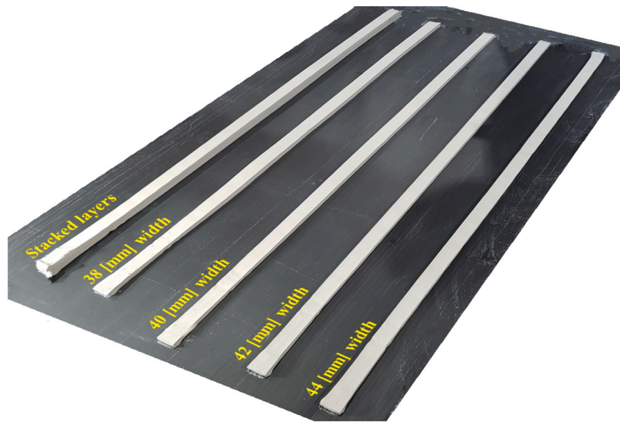
Fig. 11. Printed layers with width of 44, 42, 40 and 38 [mm] and two stacked layers.
