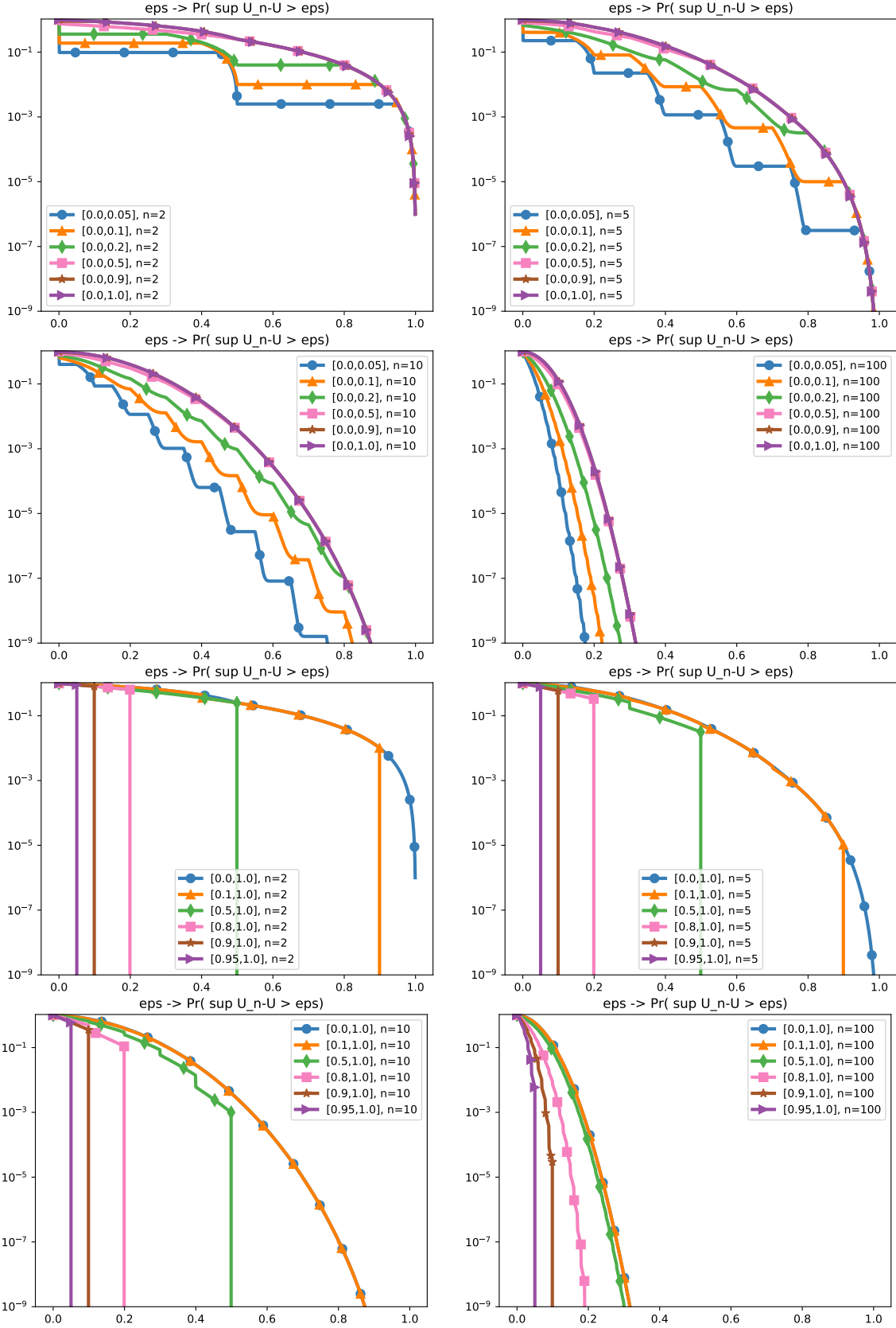
Figure 2: Plot of \varepsilon \rightarrow \delta_{[u, \bar{u}]}(n, \varepsilon) for various values of n and interval [u, \bar{u}] .
