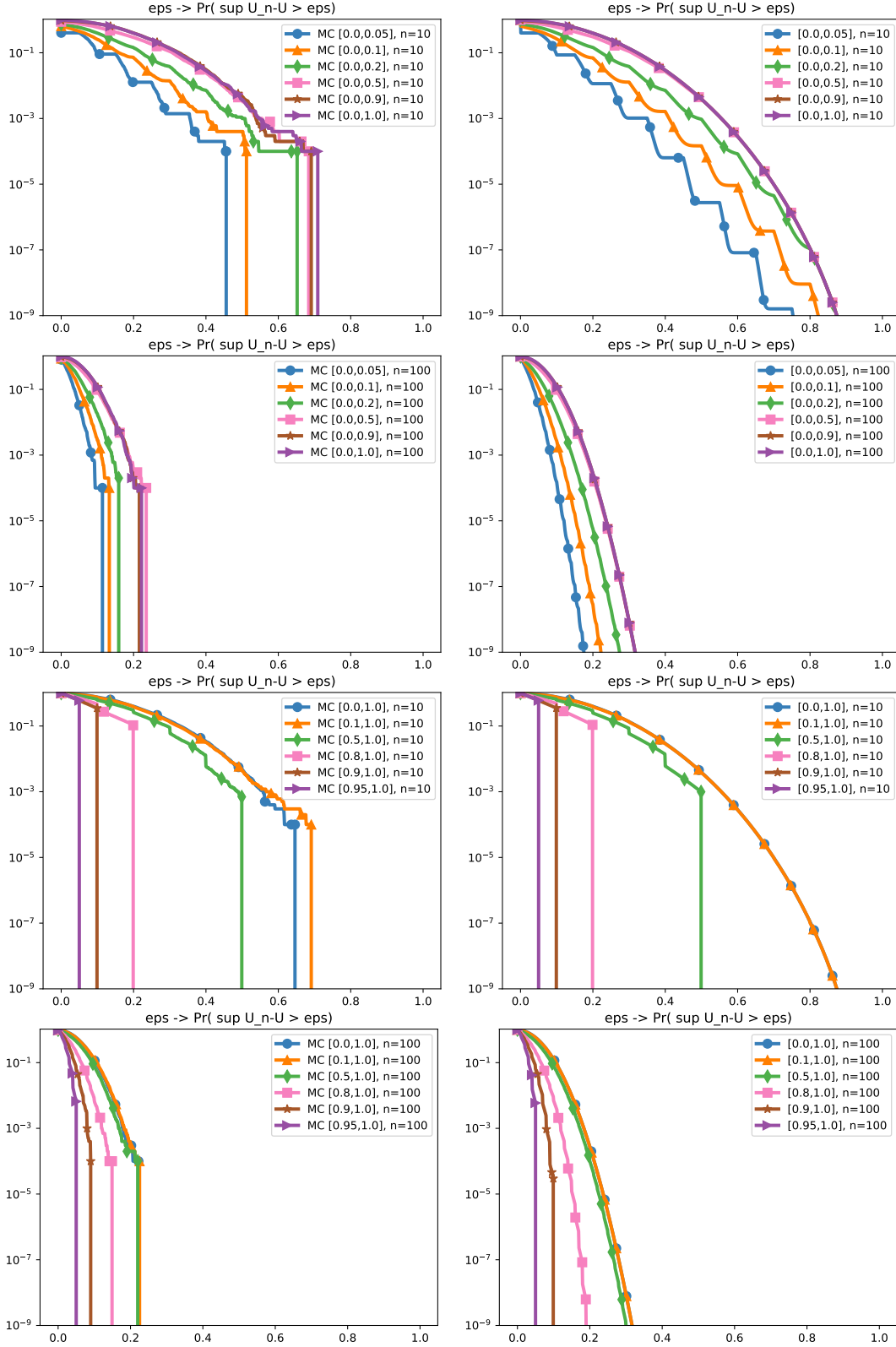
Figure 6: MCMC (left) versus Exact (Right) plot of \varepsilon \rightarrow \delta_{[\underline{u}, \bar{u}]}(n, \varepsilon) for various values of n and interval [\underline{u}, \bar{u}] build from M = 10^4 replicate.
