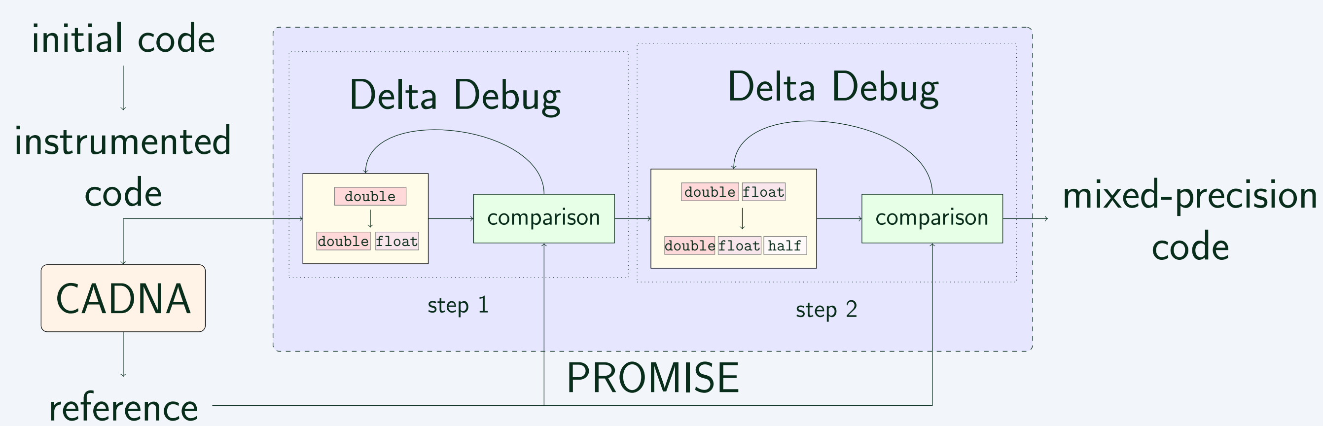
Figure 2. PROMISE Dataflow
