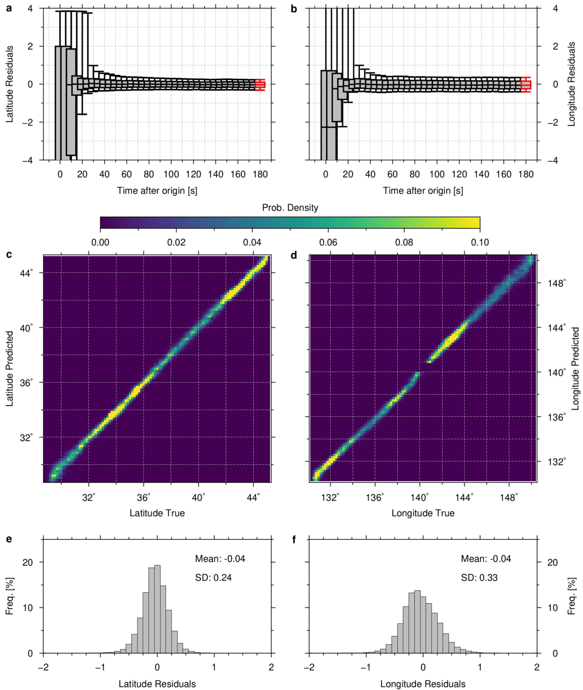
Extended Data Fig. 3 | Results of predictions on the test set for location.
