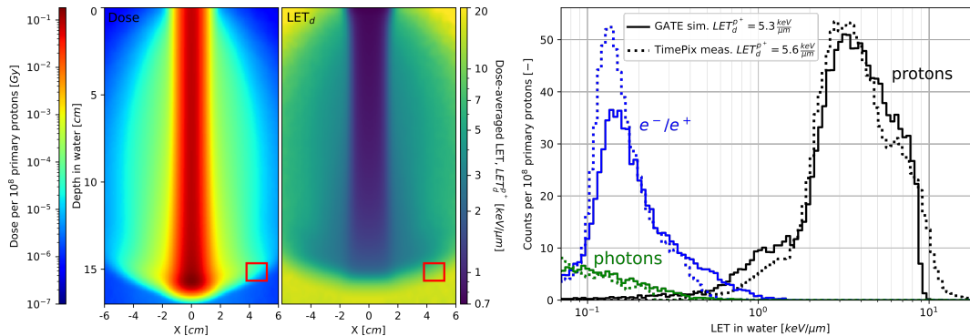
Figure 7. 2D dose (left panel) and LET_d of protons (middle panel) distributions in water for therapeutic pencil proton beam at 150 MeV and the corresponding LET spectrum (right panel) for the measurement point at the Bragg peak depth, 45 mm from the beam axis, indicated with red squares on left and middle panels. Proton, electron and photon contributions to the LET spectrum are calculated with GATE and compared to the measurement with a TimePix detector. Wide range of proton LET values is approximated by the averaged LET_d given in the legend.
