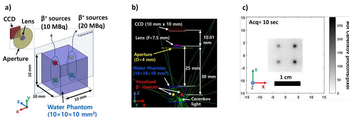
Figure 6. a) GATE Cerenkov luminescence imaging setup with optical imaging system and positron sources inside a water phantom, b) GATE Cerenkov luminescence imaging simulation geometry, c) the CCD image that collected Cerenkov luminescence light for 10 seconds.
