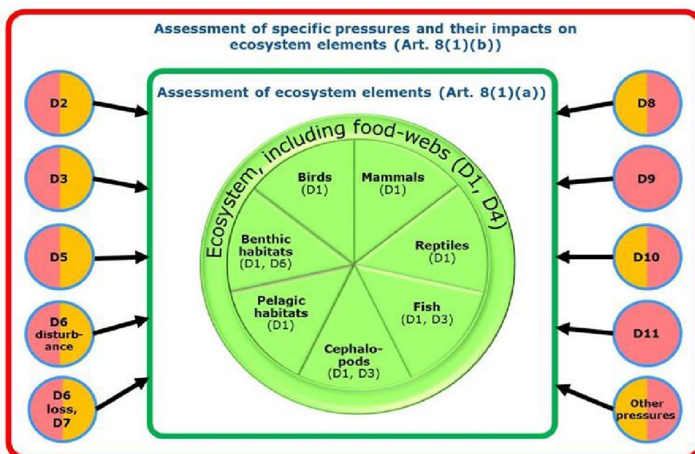
Figure 2-1: An ecosystem-based approach to determination and assessment of GES follows the main elements of the ecosystem (state-based Descriptors, centre, green) and is closely linked to the adverse effects of pressures from human activities via their environmental impacts (pressure-based Descriptors, satellite circles, in which pink depicts pressure and orange the impact). Note in relation to the satellite circles that Descriptors D2, D3, D5, D6, D7, D8 and D10 include both pressure (pink) and impact (orange) criteria in the GES Decision. For D11, impact criteria are not yet available. Source: SWD(2020) 62 final
