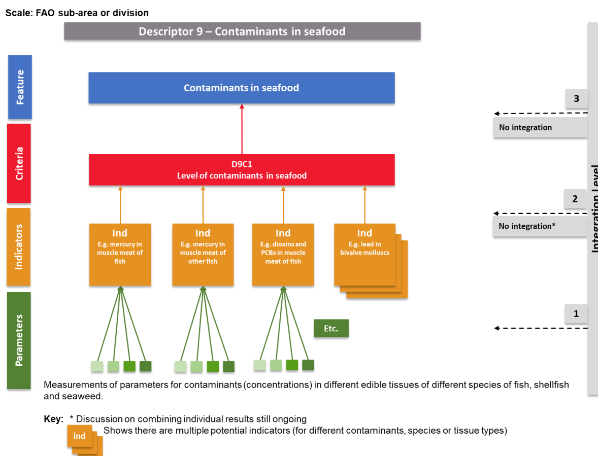
Figure 4.5-1: Levels of assessment and integration for D9.
