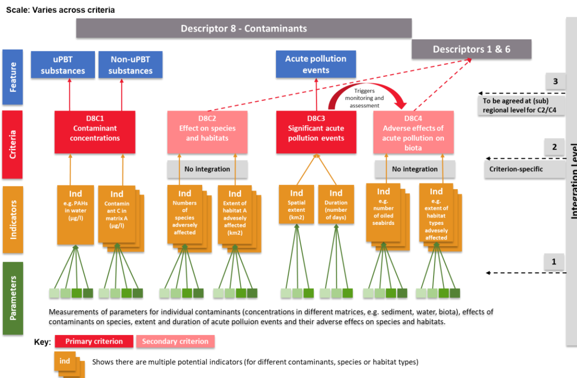
Figure 4.4-1: Use of D8 criteria and levels of integration.
