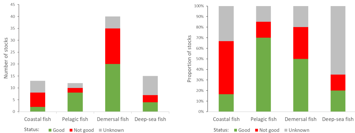
Figure 5.5-2: Examples to visualise the assessment results under D3 on stock status (based on criteria D3C1 and D3C2) per fish species group). Stock status: red – not good; green – good; grey – unknown
