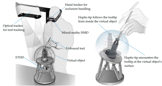
Fig. 4: Simulator using a custom haptic device based on an electric actuated hexapod [15]
