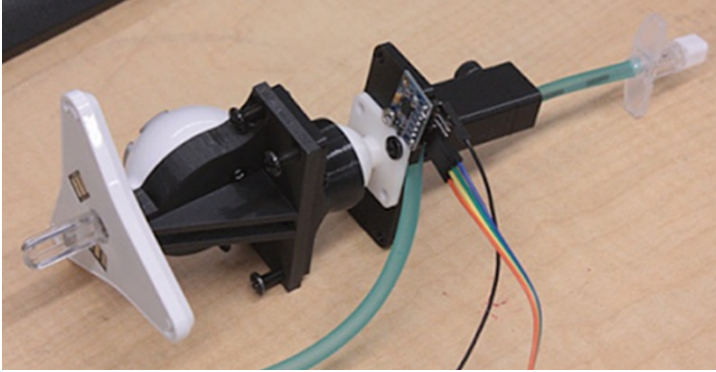
Fig. 2: Epidural simulator based on a Novint Falcon [11]
