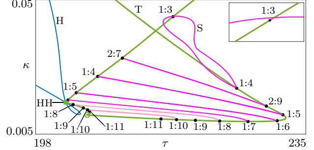
Figure 5: Bifurcation diagram in the (\tau, \kappa) -plane for A = 2.42 near the leftmost Hopf-Hopf bifurcation point HH (green dot), showing the self-intersecting Hopf bifurcation curve H (blue), the emerging pair of torus bifurcation curves T (green), and curves S (magenta) of saddle-node bifurcations of periodic orbits that bound resonance tongues arising from selected resonance points (black dots); the open circle on the lower curve T indicates the minimum of the rotation number. Curves S near this minimum that bound resonance tongues that connect two p:q resonance points are shown in lighter magenta. The inset is an enlargement near the 1:3 point.
