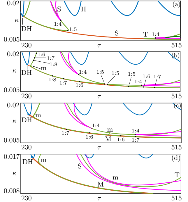
Figure 8: Disconnecting 1:4 resonance tongues of (1) in the relevant region of the (\tau, \kappa) -plane, showing the relevant bifurcation curves for A = 2.29 (a), A = 2.2605 (b), A = 2.25 (c), and A = 2.23 (d); compare with Figure 7.
