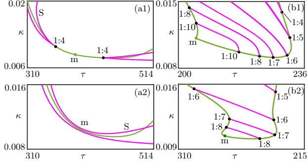
Figure 10: Disconnecting (a) and disappearing (b) resonance tongues in the (\tau, \kappa) -plane of (1) near a minimum m of the rotation number on the torus bifurcation T ; here A = 2.25 with m = 0.234 (a1), A = 2.23 with m = 0.257 (a2), A = 2.42 with m = 0.032 (b1), and A = 2.46 with m = 0.104 (b2). Compare panels (a) with Figure 8(c)–(d) and panels (b) with Figure 5.
