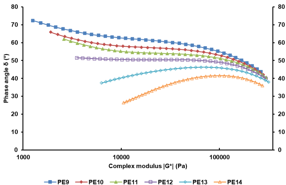
Figure 3. Rheological properties of P9-PE14 : van Gorp-Palmen plot. Shear strain ( \gamma ) 10%, angular frequencies ( \omega ) from 0.1 to 250 \text{rad}\cdot\text{s}^{-1} , T = 190\text{ }^\circ\text{C} , \text{N}_2 atmosphere.
