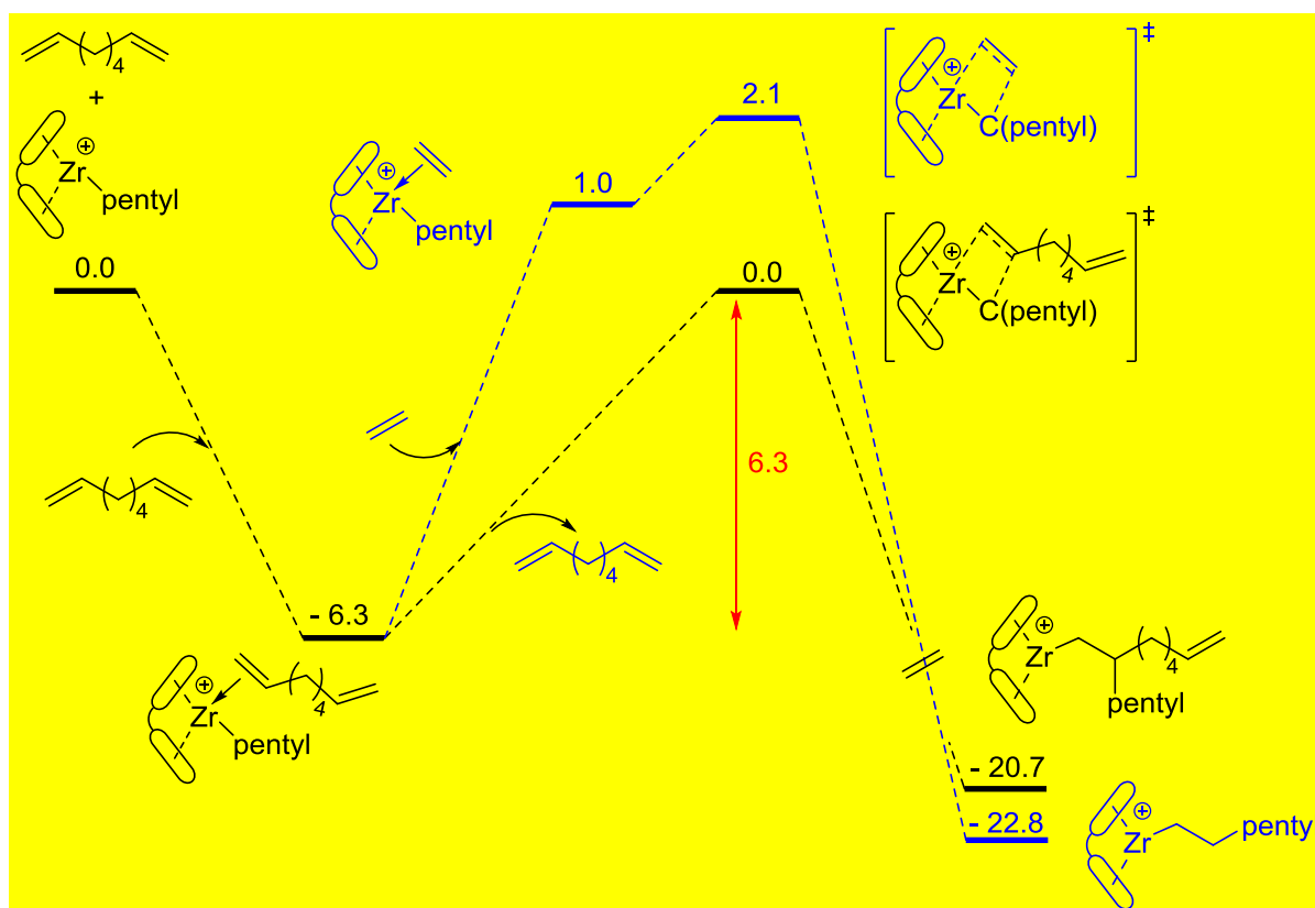
Scheme 2. A comparison between the third insertion of ethylene monomer vs. 1,7-octadiene vinyl group coordination/insertion to [\text{Zr-1-pentyl}]^+ following a dissociation of the diene.
