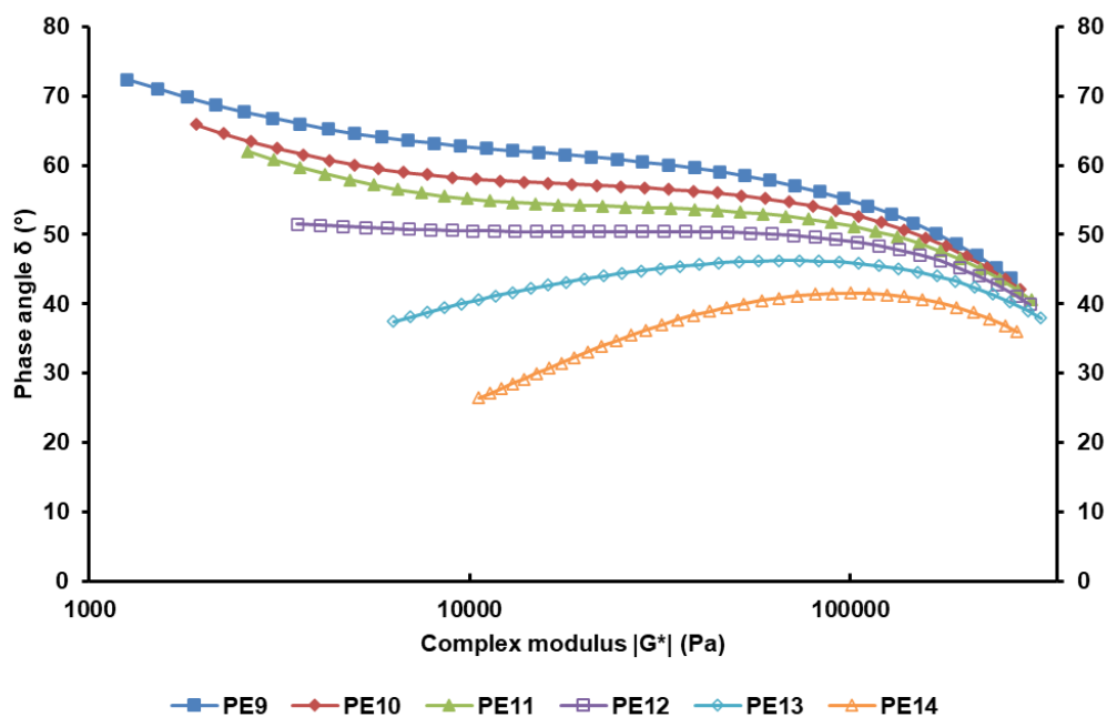
Figure 3. Rheological properties of P9-PE14 : van Gorp-Palmen plot. Shear strain ( \gamma ) 10%, angular frequencies ( \omega ) from 0.1 to 250 \text{rad}\cdot\text{s}^{-1} , T = 190\text{ }^{\circ}\text{C} , \text{N}_2 atmosphere.
