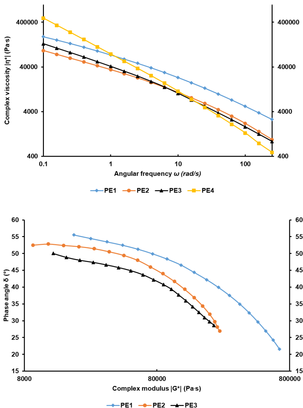
Figure 1. Rheological properties of PE1–PE4 : |\eta^*| = f(\omega) (top), van Gorp-Palmen plot (bottom, no PE4 shown [39]). Shear strain ( \gamma ) 10%, angular frequencies ( \omega ) from 0.1 to 250 \text{rad}\cdot\text{s}^{-1} , T = 190^\circ\text{C} , \text{N}_2 atmosphere.
