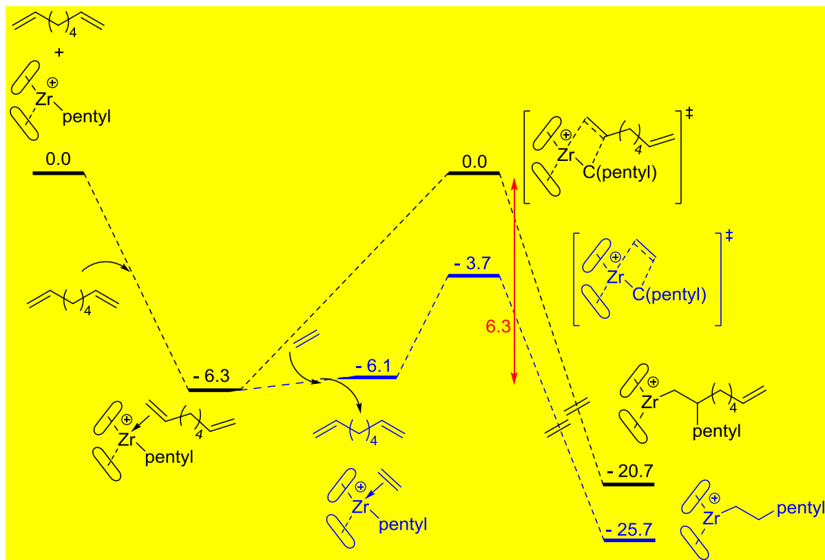
Scheme 3. A comparison between the third insertions of ethylene monomer vs. 1,7-octadiene vinyl group coordination/insertion in [\text{Zr-2-pentyl}]^+ .
