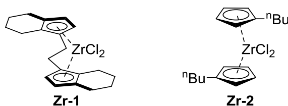
Chart 1. Structure of the metallocenes used in this study: rac -{EBTHI}ZrCl 2 ( Zr-1 ) and ( n BuCp) 2 ZrCl 2 ( Zr-2 ).
