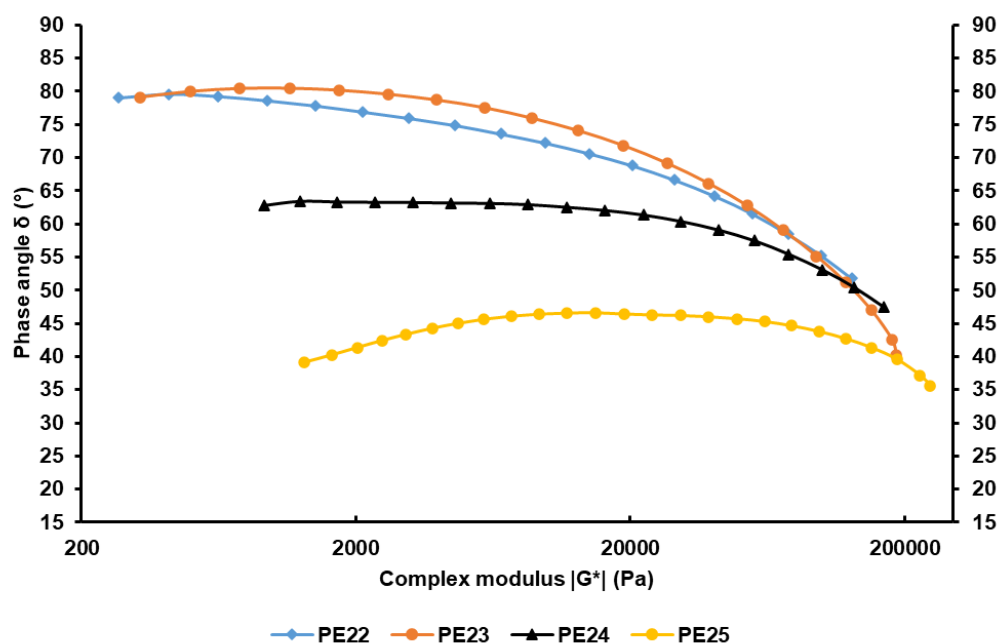
Figure 5. van Gorp-Palmen plot for the PEs obtained with supp-Zr-1 /TIBAL/1,7-octadiene mixtures – Effect of the reaction time. Shear strain ( \gamma ) 10%, angular frequencies ( \omega ) from 0.1 to 250 \text{rad}\cdot\text{s}^{-1} , T = 190\text{ }^\circ\text{C} , \text{N}_2 atmosphere.
