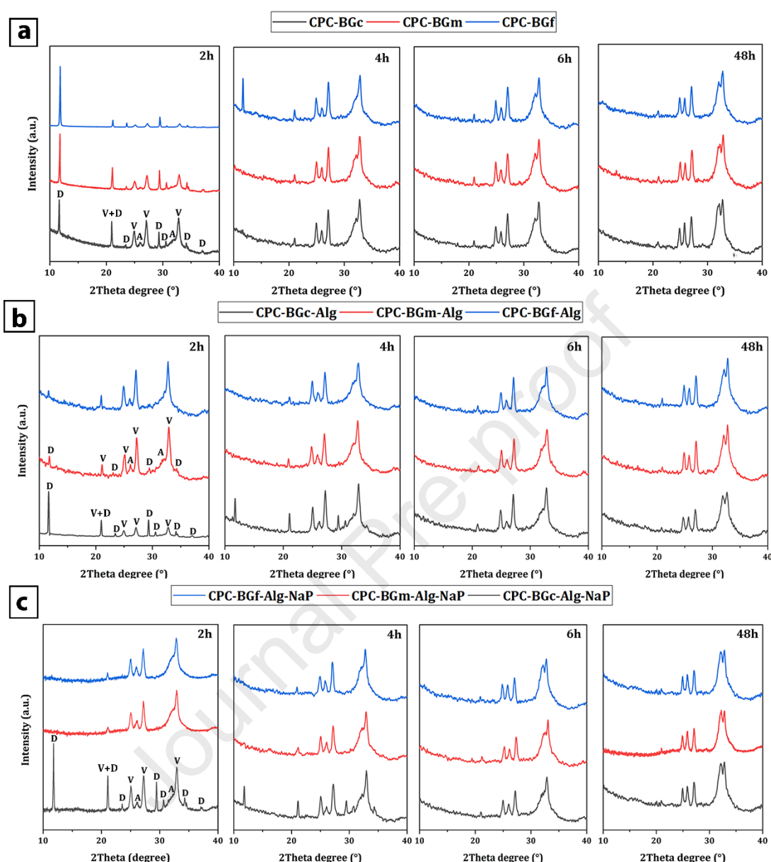
Figure 3. XRD patterns of the formulated materials as a function of reaction time, in distilled water (a), in alginate hydrogel (b), and alginate with NaP (c); (D: DCPD, V: \text{CaCO}_3 and A: Apatite)
