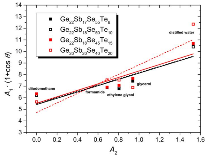
Figure 6. Owens–Wendt plot for GSST thin films on silicon wafer with indicated nominal composition
