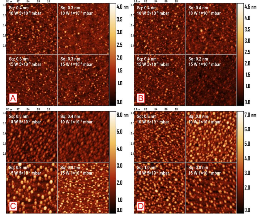
Figure 2. AFM scans of 1 \times 1 \mu\text{m}^2 area of sputtered GSST thin films (with thickness of 800 nm) with indicated RMS roughness ( Sq , \pm 0.1 nm), values on z-axis are normalized for each target nominal composition; A – \text{Ge}_{19}\text{Sb}_{17}\text{Se}_{59}\text{Te}_{5.0} , B – \text{Ge}_{19}\text{Sb}_{17}\text{Se}_{54}\text{Te}_{10} , C – \text{Ge}_{19}\text{Sb}_{17}\text{Se}_{49}\text{Te}_{15} , D – \text{Ge}_{19}\text{Sb}_{17}\text{Se}_{44}\text{Te}_{20} .
