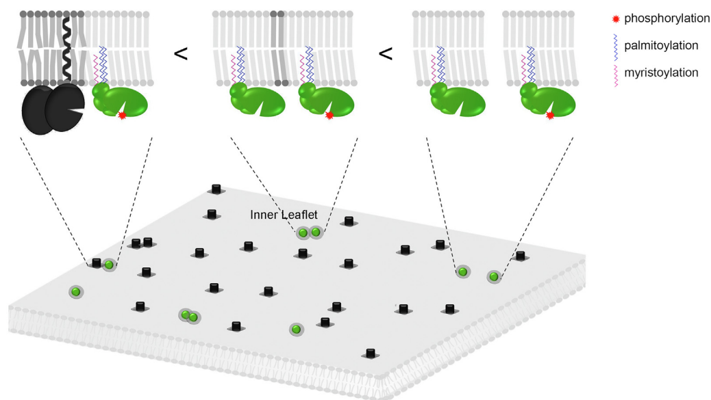
Figure 6. Schematic depiction of lateral proximity of Lck and CD45 dependent on lipid fingerprint. Specific boundary lipids codiffusing with the membrane anchor the “lipid fingerprint” of each protein. Different boundary lipids create energetic barriers that reduce the probability of lateral proximity. Bottom, Identical boundary lipids (light gray circle surrounding Lck - green) favor Lck \leftrightarrow Lck interaction. Different annular lipids (dark gray squares surrounding CD45 - black) do not veto CD45 \leftrightarrow Lck interaction but make it less favorable. CD45 \leftrightarrow CD45 interaction may be functionally inconsequential. (Top) “Lipid fingerprints” for CD45 and Lck are idealized by lipids of different aliphatic chain length and/or saturation but can be further diversified by hydrophobic mismatch and charged lipid heads.
