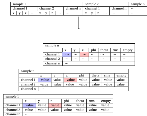
Figure 5: Scheme of the reshaping of the data array into two-dimensional matrices per sample. Colored cells represent positions in the horizontal dimension (blue) and the vertical dimension (red) for each sample.
