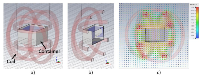
Fig. 1. Test bench design using CST Studio Suite: global overview (a), sectional view (b) and magnetic field distribution (c)
