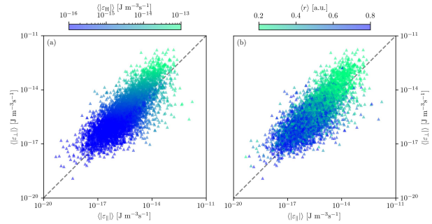
Fig. 5. Cascade rate component \langle \varepsilon_{\perp} \rangle as a function of the component \langle \varepsilon_{\parallel} \rangle . In panel a the color bar is the total cascade \langle \varepsilon_H \rangle (where \varepsilon_H = \varepsilon_{\perp}/2 + \varepsilon_{\parallel}/4 is the total hybrid cascade rate), and in panel b it is the heliocentric distance \langle r \rangle .
