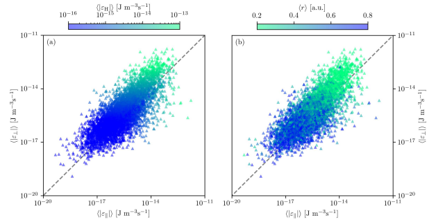
Fig. 5. Cascade rate component \langle \varepsilon_{\perp} \rangle as a function of the component \langle \varepsilon_{\parallel} \rangle . In panel a the color bar is the total cascade \langle \varepsilon_H \rangle (where \varepsilon_H = \varepsilon_{\perp}/2 + \varepsilon_{\parallel}/4 is the total hybrid cascade rate), and in panel b it is the heliocentric distance \langle r \rangle .
