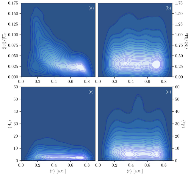
Fig. 3. Bivariate KDE for the normalized fluctuation ( a and b ) and variance anisotropy ( c and d ) ratios respectively for the velocity and magnetic fields as a function of the heliocentric distance. The dotted lines in panels c and d correspond to the isotropic (kinetic or magnetic) energy distribution.
