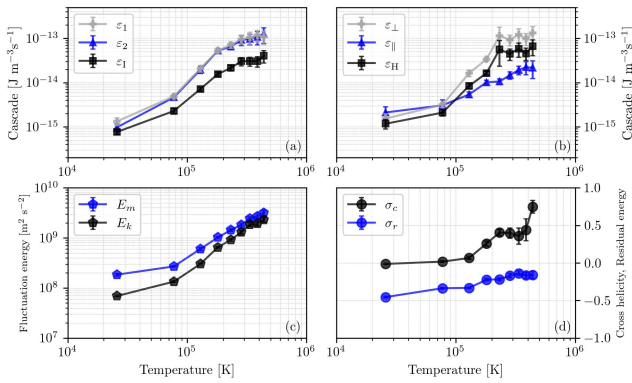
Fig. 7. For a given temperature bin the following averages are shown: (a) Components and total isotropic energy cascade rates; (b) components and total anisotropic energy cascade rates; (c) fluctuation in kinetic and magnetic energies; and (d) normalized cross-helicity and normalized residual energy as a function of the temperature.
