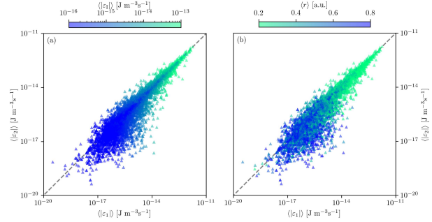
Fig. 4. Cascade rate component \langle \varepsilon_2 \rangle as a function of the component \langle \varepsilon_1 \rangle . In panel a the color bar is the total cascade \langle \varepsilon_1 \rangle , and in panel b it is the heliocentric distance \langle r \rangle .
