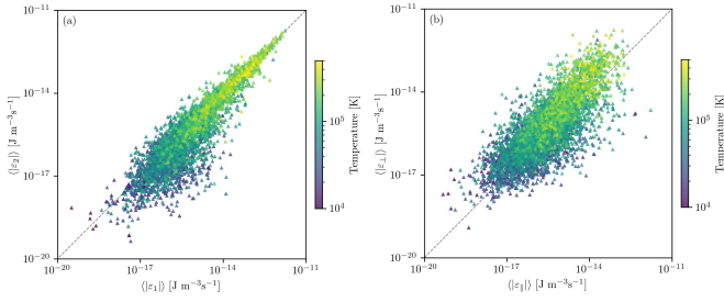
Fig. 6. Cascade rate component \langle \varepsilon_2 \rangle as a function of the component \langle \varepsilon_1 \rangle , and the perpendicular component \langle \varepsilon_{\perp} \rangle as a function of the parallel component \langle \varepsilon_{\parallel} \rangle . In panels a and b the color bar is the temperature.
