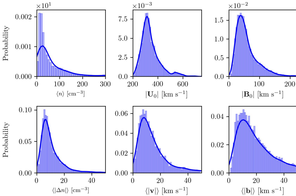
Fig. 1. Occurrence rates for the proton density, and the proton and Alfvén velocity absolute mean values ( top ) and fluctuations ( bottom ).
