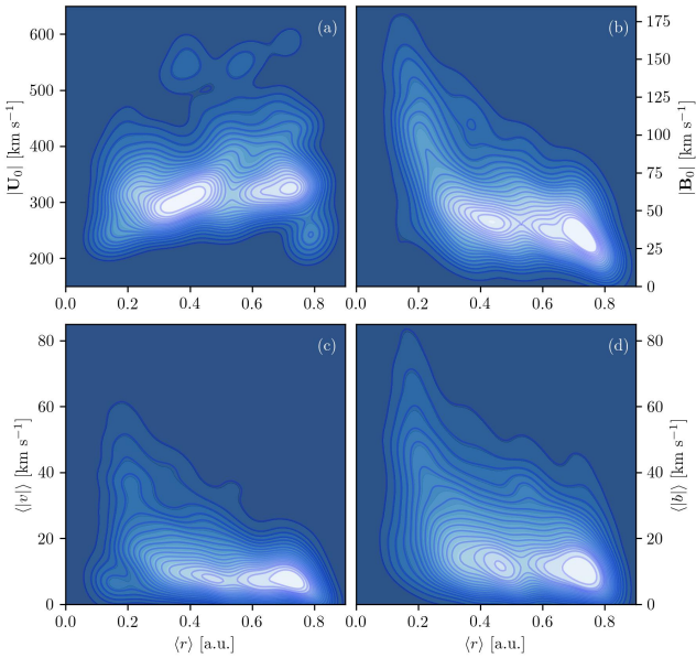
Fig. 2. Bivariant KDE for the mean ( a and b ) and fluctuating ( c and d ) velocity and magnetic field absolute values as a function of the heliocentric distance.
