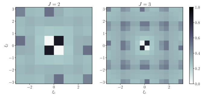
Fig. 5. Relative quadratic error between the outputs of \mathbb{R}G\text{Pool} and \mathbb{C}G\text{Mod} . For each wavelet packet channel l \in \{0 \dots L_J - 1\} , (\tilde{\rho}_l^{(J)})^2 is represented as a grayscale pixel centered in \xi_l^{(J)} , such as introduced in (86). Since the subsampling factor m_J is equal to 2^{J-1} , these empirical estimates can be compared with the left and right parts of Fig. 4. The plots are symmetrized to account for the complex conjugate feature maps.
