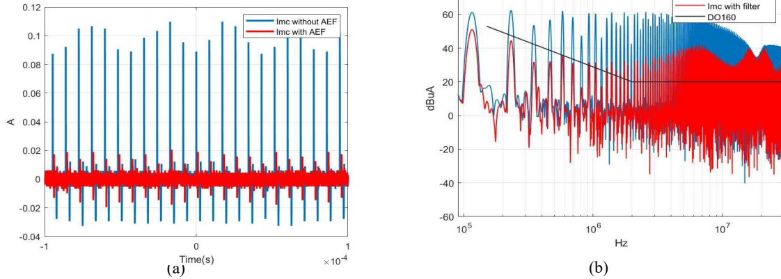
Fig 11a: Comparison between Imc with filter and without filter, (b) Comparison between common mode noise spectrum with and without filter
