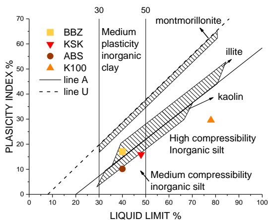
Fig. 3 Plasticity chart
