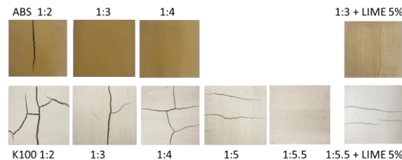
Fig. 6 Shrinkage test.
