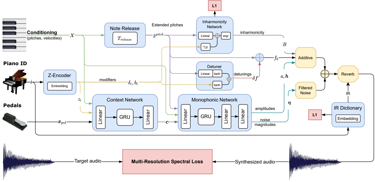
Figure 1: Full architecture of the proposed piano sound synthesizer. The blue boxes represent the trained modules for the control of the synthesis. The synthesis modules from DDSF are represented by yellow boxes (Additive, Filtered Noise, and Reverberation). Finally, the Multi-Resolution Spectral Loss compares the input target signal (bottom left) and the output synthesized sound (bottom right).
