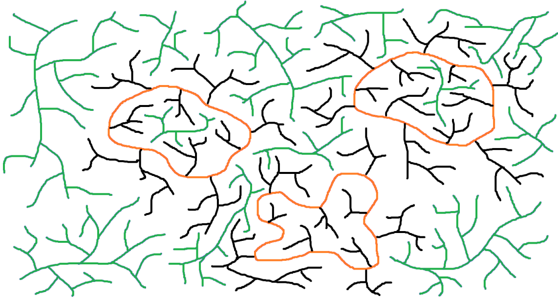
FIGURE 12. Conceptual depiction of the sign clusters of the metric GFF in high dimension. The trees are not exactly so, but are actually made of microscopic loops at the metric graph level. Most large clusters are macroscopically tree-like, as the trees in green. Their number diverges in the scaling limit. However, there is a tight number per scale of macroscopic cycles, that are represented in orange. The limit distribution of the macroscopic cycles is that of a Brownian loop soup of intensity parameter \alpha = 1 , that is to say double of the intensity appearing in isomorphism theorems.
