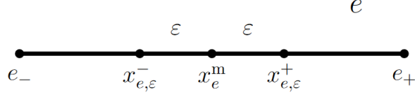
FIGURE 7. Inside an edge-line.
