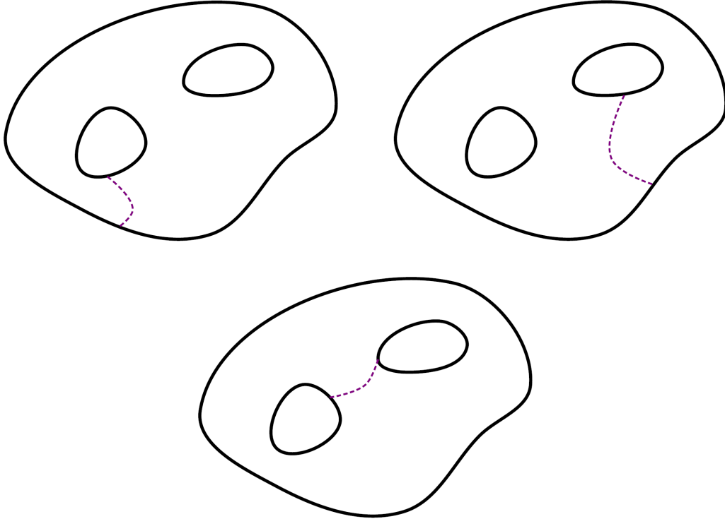
FIGURE 10. Depiction of 3 non-equivalent gauge fields on a planar domain with 2 holes. The defect lines are in violet dashed.
