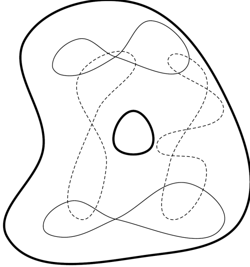
FIGURE 6. A non-contractible chain in an annular domain formed by contractible loops.
