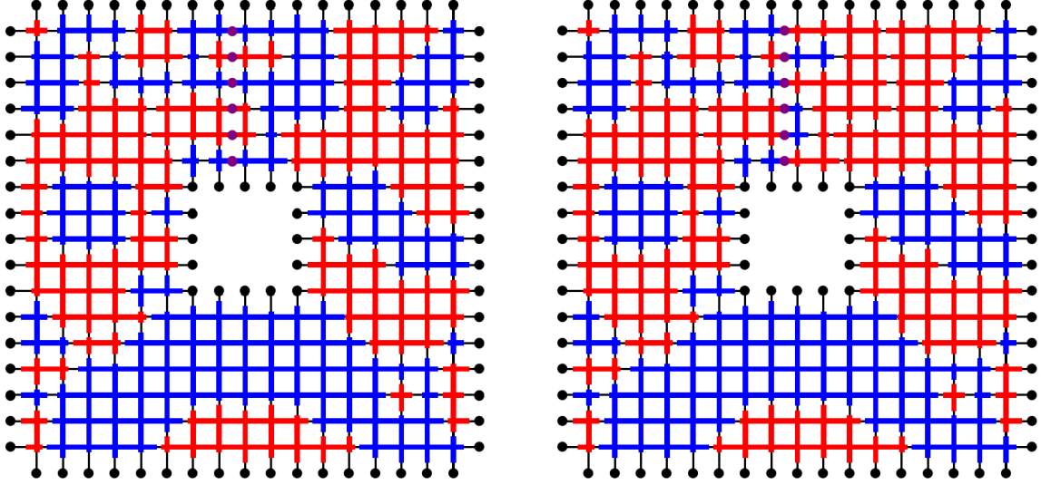
FIGURE 8. Left: the field \tilde{\phi} on the event \tilde{\phi} \in \mathcal{T}_\sigma , which in this example means that there are no sign clusters surrounding the inner hole of the domain. Right: the associated \tilde{\xi} field. The black dots represent the boundary V_\partial . The violet dots represent \mathfrak{M}_\sigma . The positive, resp. negative values of the fields are in red, resp. blue.
