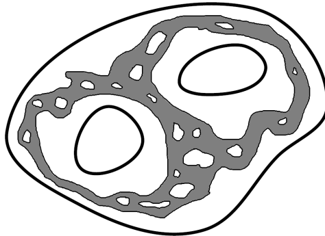
FIGURE 11. Depiction in grey of a cluster that is non-trivial for simultaneously all the 3 defect lines on Figure 10.
