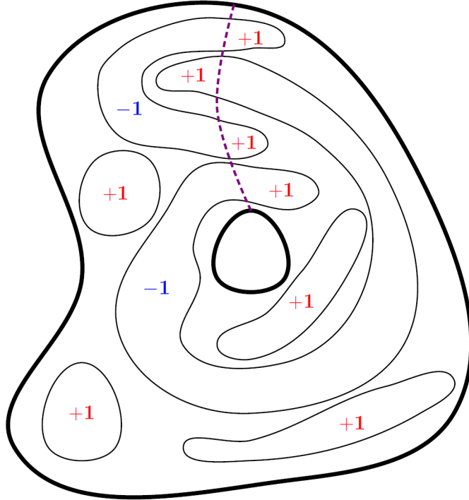
FIGURE 9. Conceptual depiction of the signs \zeta_{\mathfrak{C},\gamma} . The defect line \gamma is represented in violet dashed.
